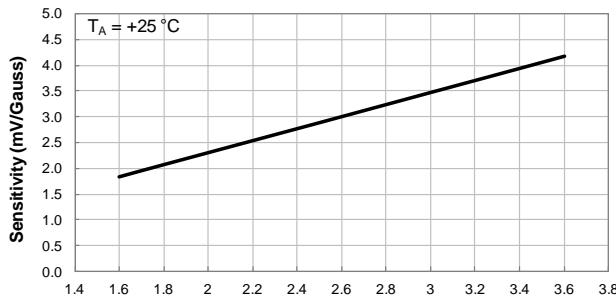
Sensitivity vs Supply Voltage
