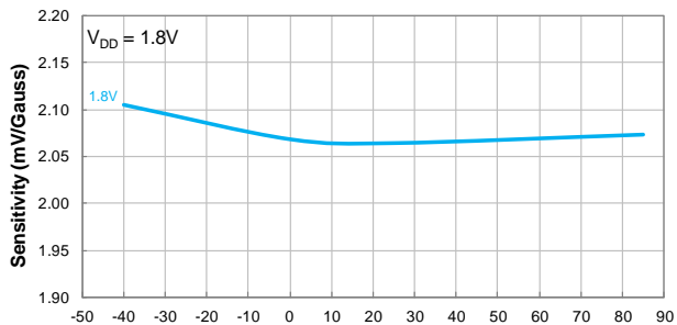
Sensitivity vs Temperature
