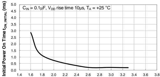
Initial Power On Time vs Supply Voltage
