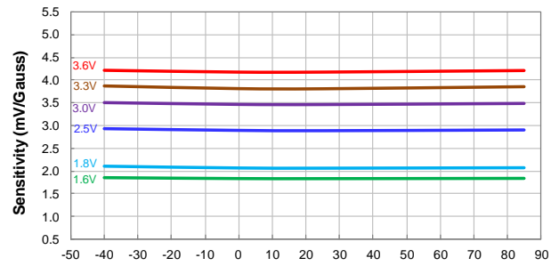
Sensitivity vs Temperature
