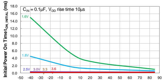
Initial Power On Time vs Temperature
